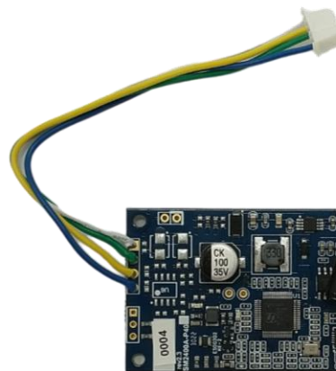
SM2400A-P40-Rev2.3 Production-Ready PLC Module
